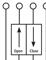
14) Connecting terminals for external buttons
